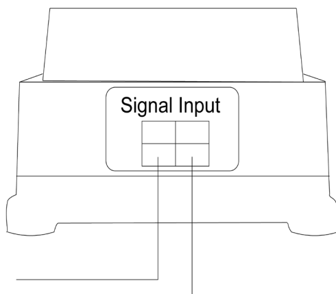
fig 8 cable to ports A/B on rear end of T-POD10XRF
