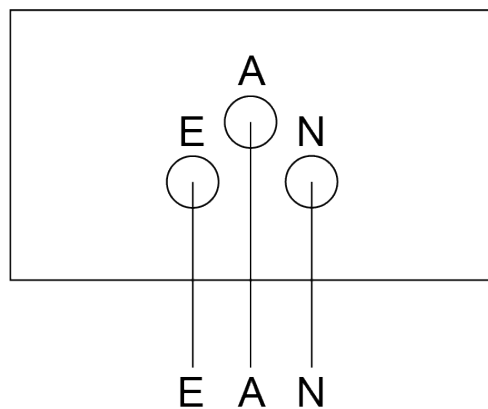
Wiring Diagram for GPO
